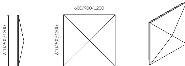
Absorber CubiSound symmetrisch
